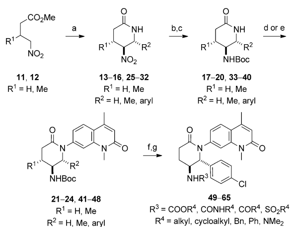
Scheme 2. Synthesis of analogues for SAR studies around the lead scaffold. Reagents and conditions: a) R^3\text{CHO} , \text{NH}_4\text{OAc} , EtOH, 90°C, 26–86%, d.r. 2:1–> 20:1; b) \text{NiCl}_2 \cdot 6\text{H}_2\text{O} , \text{NaBH}_4 , MeOH, 0°C; c) \text{Boc}_2\text{O} , 39–91% (2 steps); d) 4 , [\text{Pd}_2(\text{dba})_3] , Xantphos, \text{Cs}_2\text{CO}_3 , 1,4-dioxane, 100°C, 2–75%; e) 4 , \text{K}_3\text{PO}_4 , CuI, (±)- trans -1,2-diaminocyclohexane, 1,4-dioxane, 97°C, 7–65%; f) HCl/dioxane, 96%; g) R^2\text{Cl} , TEA, \text{CH}_2\text{Cl}_2 or \text{RNCO} , \text{CH}_2\text{Cl}_2 , 12–60%. Boc = tert -butoxycarbonyl, TFA = trifluoroacetic acid.
